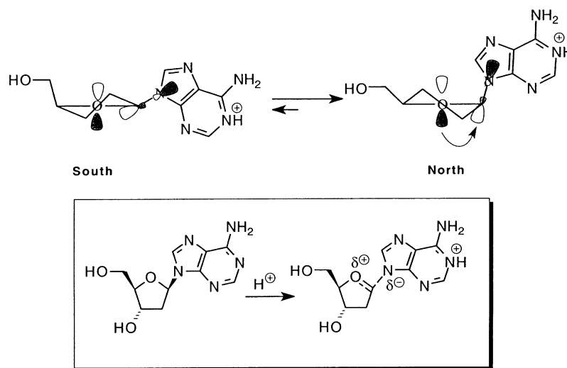
Figure 1. O4'–C1'–N9 anomeric effect. The lone pair orbitals are sp^2 [higher energy 1n_{sp}^2 (p-type), lower energy 2n_{sp}^2 (s-type)]. The n_{O4'} \rightarrow \sigma^* overlap stabilizes the North conformation following protonation of the base (box). 23 Orbital interaction in the North conformation is possible due to a near anti-periplanar orientation.
